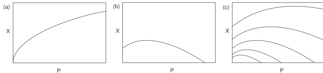
FIGURE 8.3. PPFs. The PPF in (a) is not allowed because there is no turning point; the PPF in (b) is allowed; in (c) we see a set of PPFs for different productivity levels.
