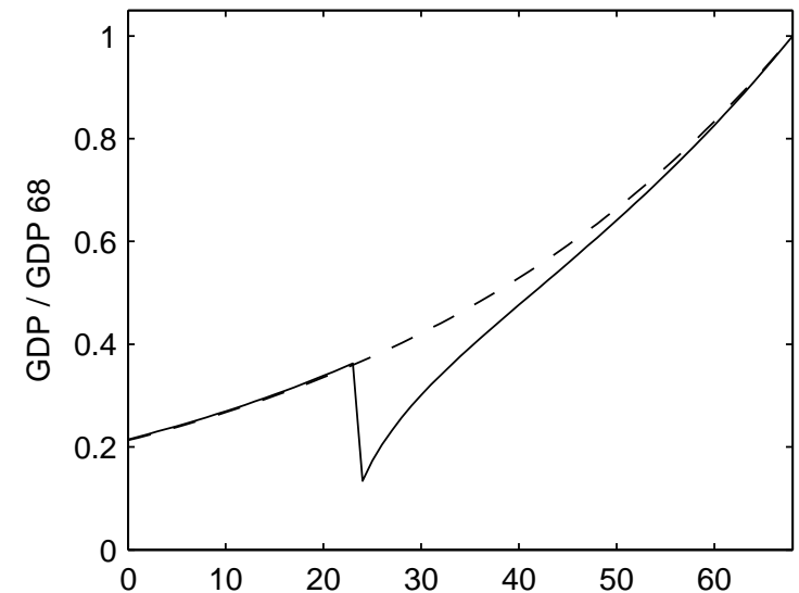
Figure 2: Testing the Solow model. Upper panel: German real GDP, compared to an estimated constant-growth trend (growth rate 2.3 percent per year). Lower panel: Model simulation assuming the same growth trend in labour productivity and parameters \alpha = 0.3 , \delta = 0.1 , s = 0.2 , with a massive shock to capital (the stock is divided by a factor of 30 at the end of year 24).
